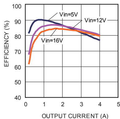
Efficiency
