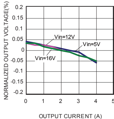
Load Regulation
